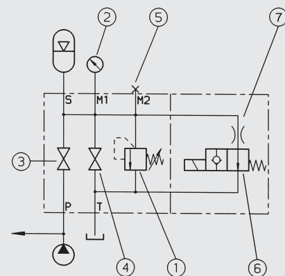
Circuit diagram
